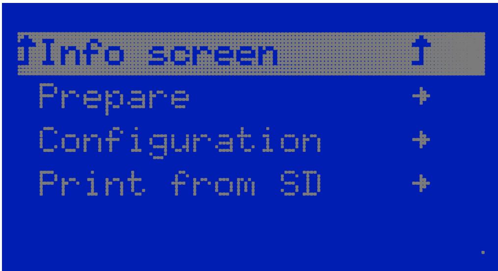
Figure 3.2: Main menu
